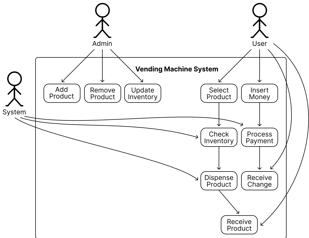
Use Case Diagram of a Vending Machine
