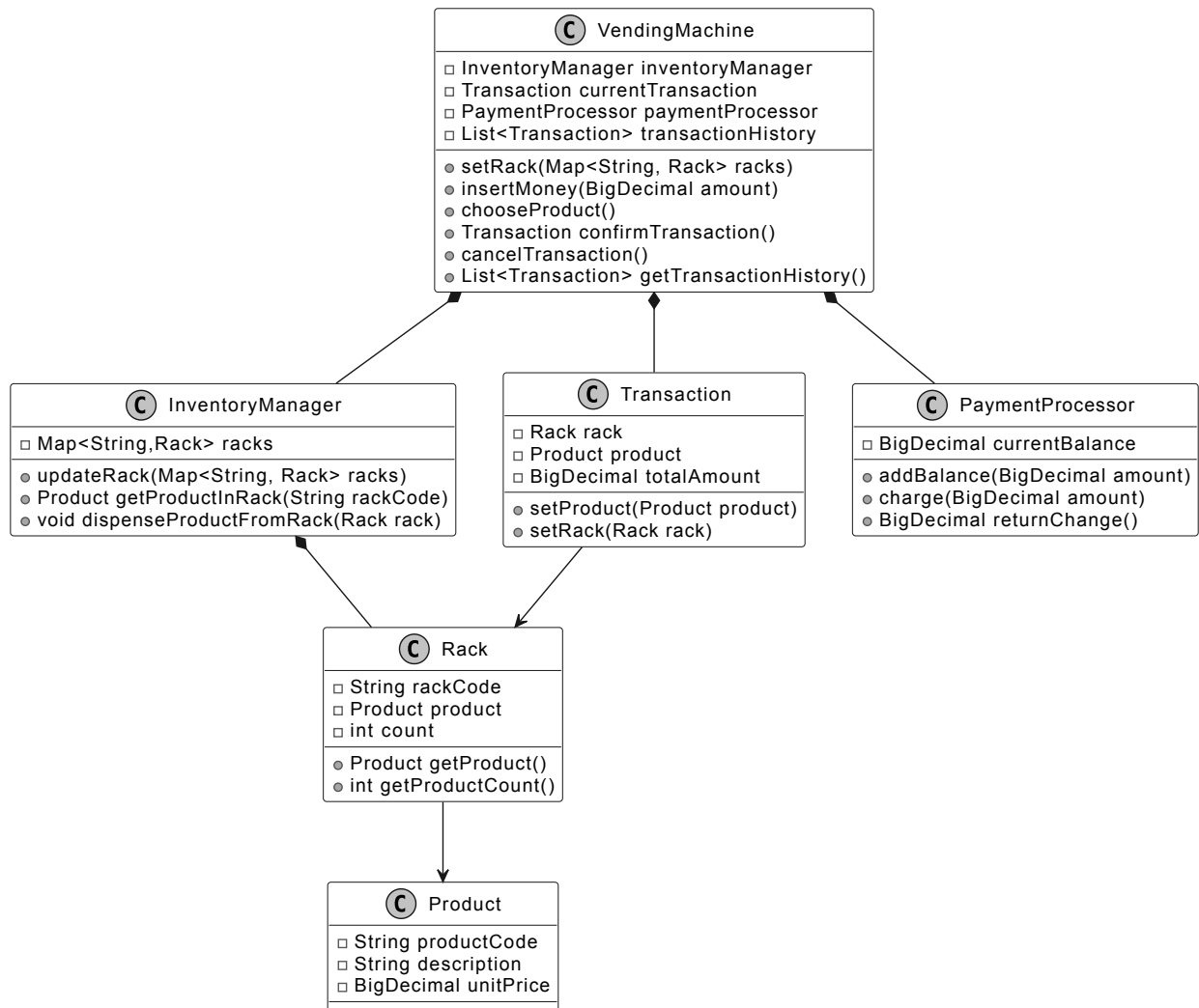
Class Diagram of Vending Machine
